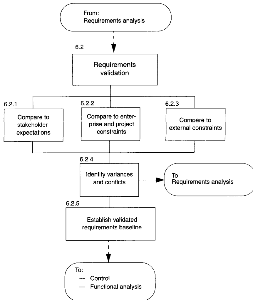
Figure 11—Requirements validation
