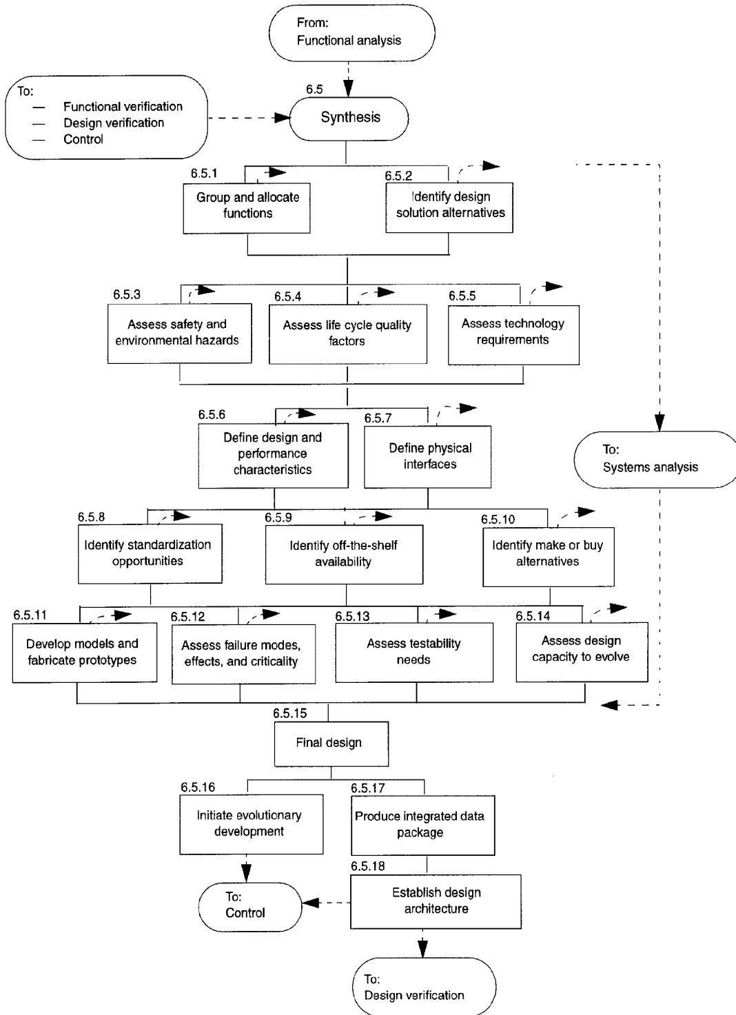
Figure 14—Synthesis process
